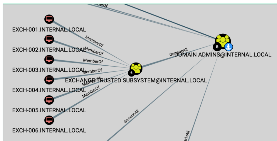
Above: A typical scenario in many enterprise networks: the Exchange Trusted Subsystem, with all Exchange computer objects as members, has full control over the Domain Admins group.
